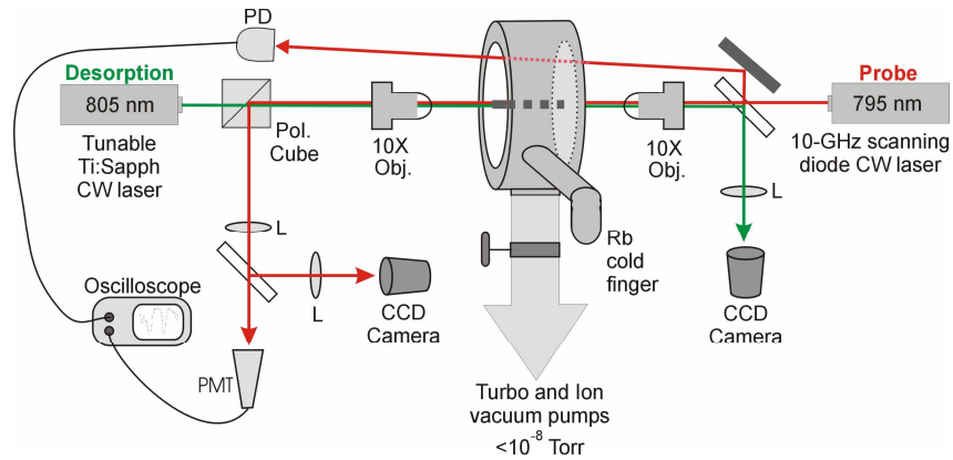
Fig. 1. A schematic of the experimental layout: A 4.5-cm-long hollow-core photonic bandgap fiber is mounted inside a steel chamber with glass windows connected to an ultrahigh vacuum system. 795-nm probe light and 805-nm atom-desorbing light are coupled into the fiber in counter-propagating geometry with 10 \times microscope objectives, and the coupling is monitored using a CCD camera. The probe beam can alternately be passed through the cell and detected by a photodiode to monitor the ambient cell Rb density. The coupled probe light is detected with photomultiplier tube (PMT). L: lens; PD: photodiode.
